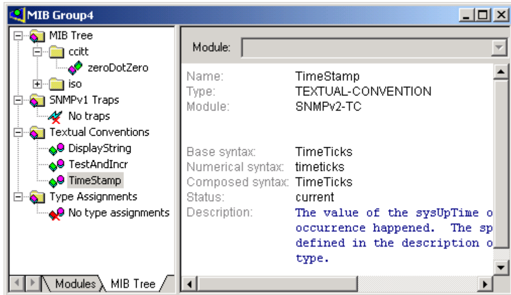
Figure 7: MIB Group window, MIB Tree tab
